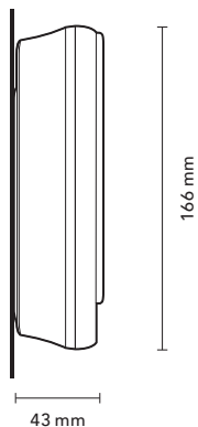
Wall mount
